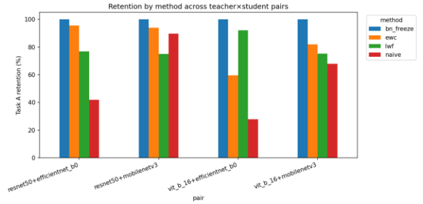
Figure 6. Task-A retention by method, grouped by teacher×student pair.
